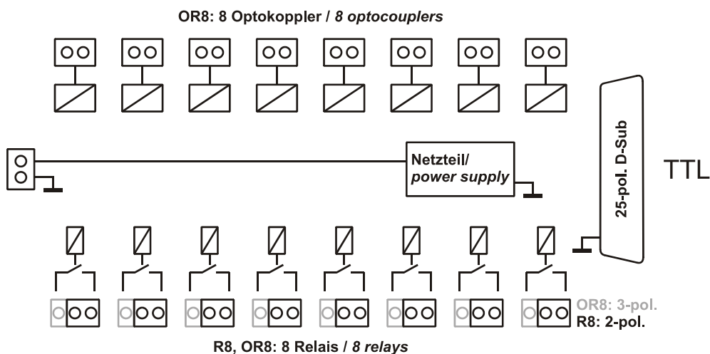
Functional diagram
