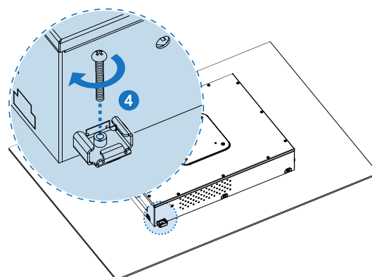
Figure 14 Panel Mounting
