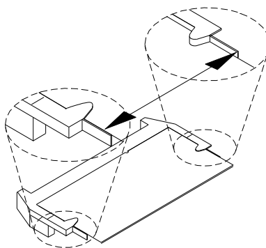
Figure 8 Press down on the SO-DIMM Memory Module to lock it in place
