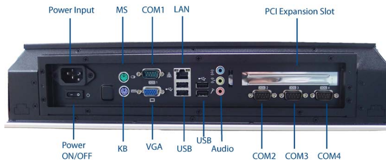
Figure 2 Mechanical Layout - I/O Panel
