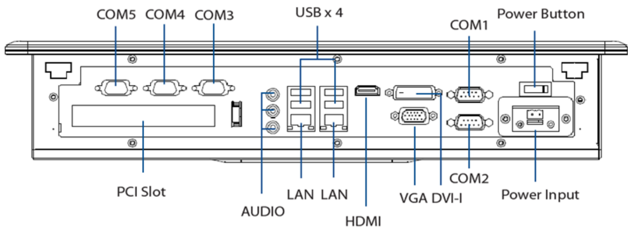
Figure 1 Rear I/O
