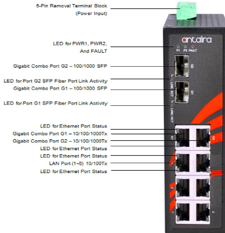
Figure 2.2 - The Front Panel of the LNX-0802C-SFP Series
