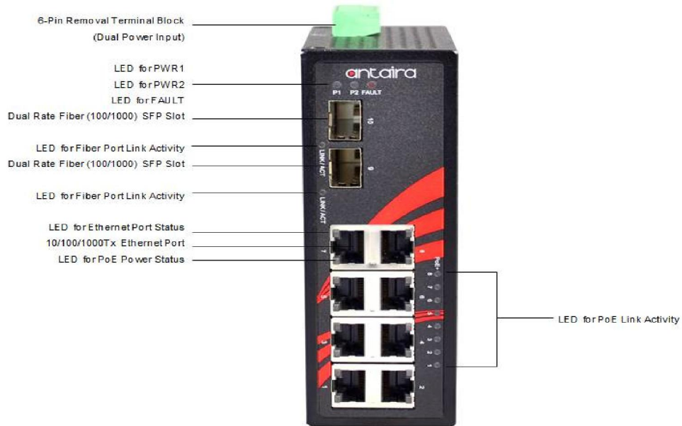
Figure 2.2 The Front Panel of LNP-1002G-SFP Series
