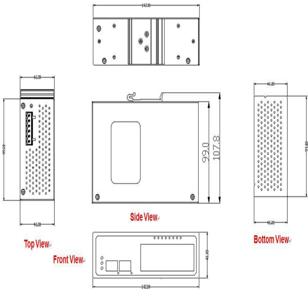
Figure 2.1 LNP-1002G-SFP Series Physical Dimensions
